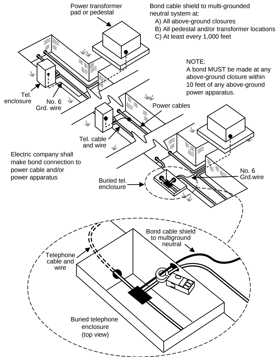
JOINT BURIED CONSTRUCTION – RANDOM SEPARATION
